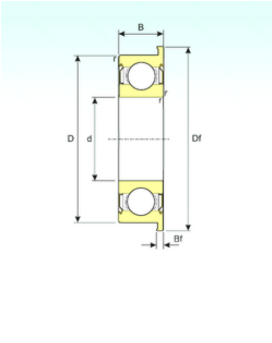
F6805ZZ Bearing 2D drawings and 3D CAD models
